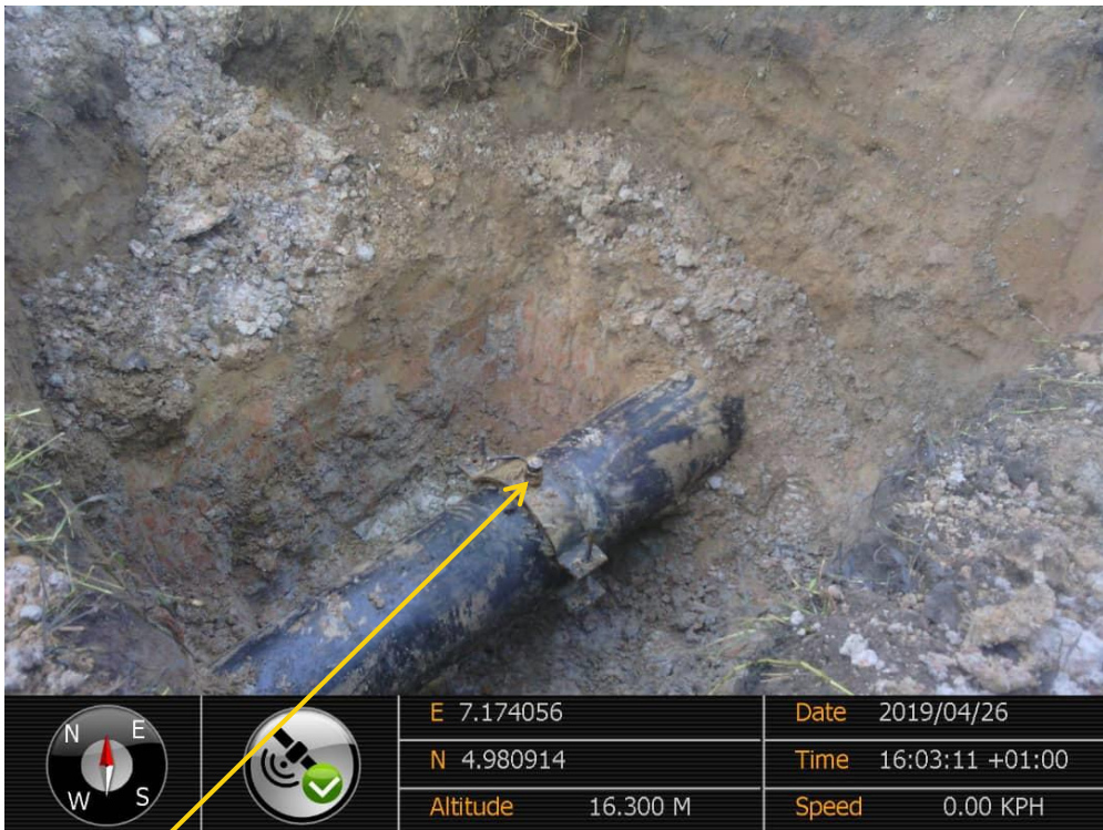
Close-up: Illegal Fitting on 12" Imo River2 – Ogale Pipeline at Igiriukwu-Owaza. Picture was taken during Joint Investigation of 26 th April 2019.
