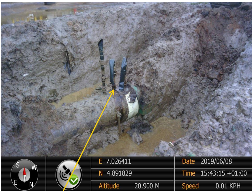
Close-up: Leaking Illegal Fitting on 28'' Nkpoku – Ogale Pipeline at Rumuowha-Eneka. Picture was taken during Joint Investigation of 8 th June 2019
